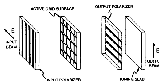
Figure 2: A grid amplifier on a dielectric slab with X and Y polarizers.
