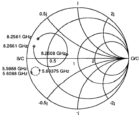
Figure 8: Impedance Smith chart showing the input impedance of the patch antenna without the reflector: solid line, simulation; dashed line, measurement.
