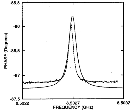
Figure 5: Input impedance phase of the L antenna for the TEM_{0,0,35} mode: solid line, simulation; dashed line, measurement.
