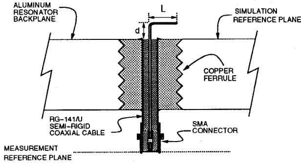
Figure 3: A coaxial fed inverted L antenna.
