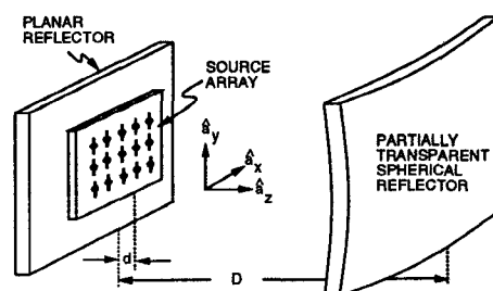
Figure 1: Quasi-optical power combiner configuration.
